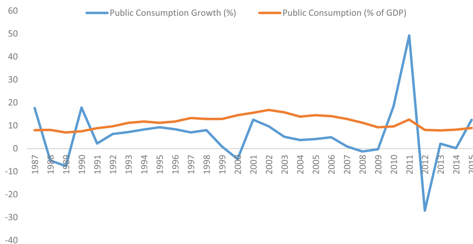
Figure 2: Public Consumption
